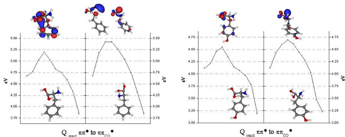
Figure 6: Potential energy profiles of the S_1 state for the proton transfer to CO reaction following the optimization of the \pi\pi_{CO}^* excited state for the stack and rot conformers of PheH + (left) and TyrH + syn (right). The starting point is the adiabatic energy of the \pi\pi^* state. The last point corresponds to the proton transferred species to the carboxylic group (structures represented at the bottom of the figures). For both molecules, the height of the barrier for the \pi\pi^*/\pi\pi_{CO}^* curve crossing is about 0.4 eV for the stack conformer and 0.6 eV for the rot structure. For each conformer, the most contributing molecular orbitals of the transition states are represented on the top of the figure.
