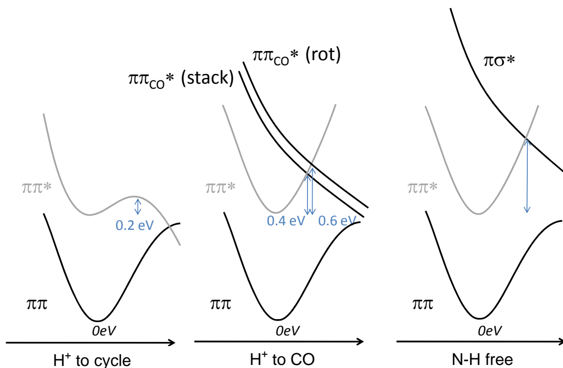
Figure 8: Schematic potential energy functions for the excited states of \text{PheH}^+ or \text{TyrH}^+ as a function of the proton transfer coordinate towards the aromatic ring (left), towards CO (middle), and versus the \text{NH}_{\text{free}} coordinate (right). The barrier heights are qualitatively indicated by blue arrows. They differ from one conformer to the other along the proton transfer to the CO.
