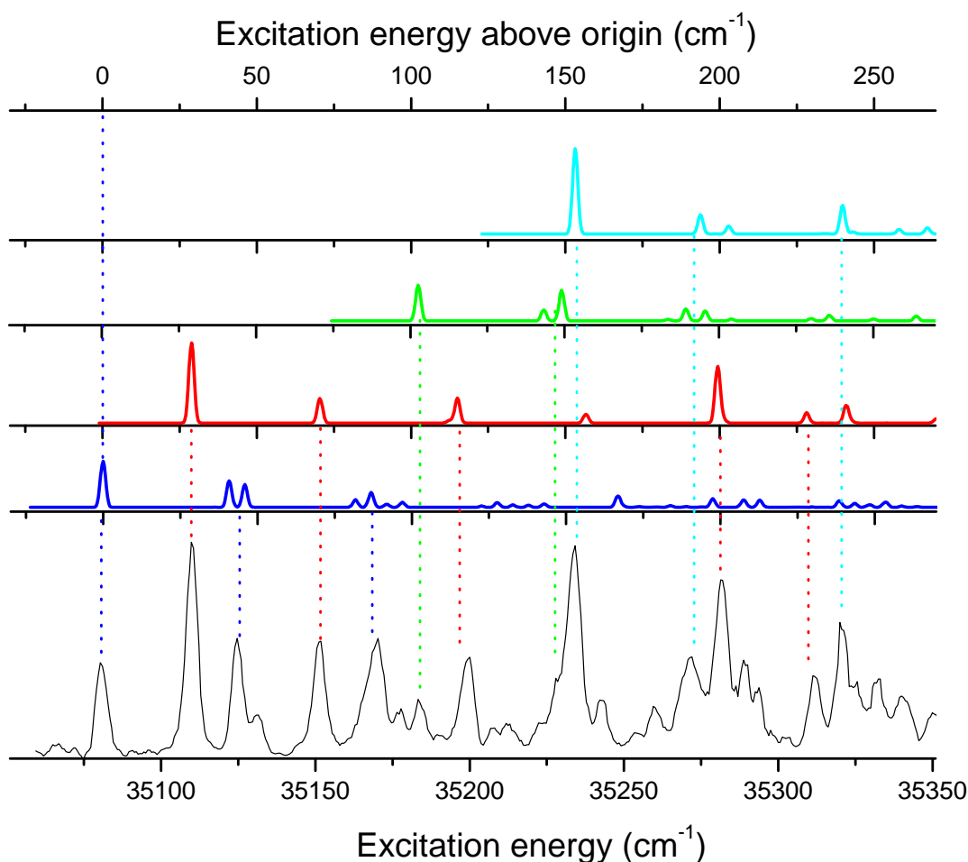
Figure 1: comparison between the experimental (recorded on the m/z 108, lower trace) and the calculated spectra (color on line: blue, stack/syn ; red, rot/syn ; green, stack/anti ; cyan, rot/anti ) of the 4 conformers of TyrH + .
