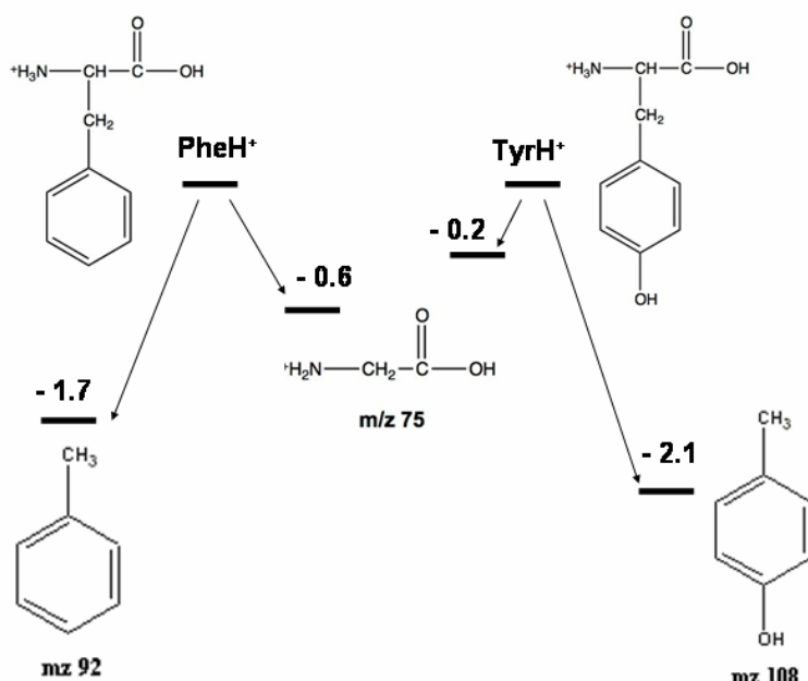
Figure 7: Calculated exothermicities (energies in eV) of C α -C β bond cleavage reactions leading to the final ionic products in PheH + and TyrH + .
