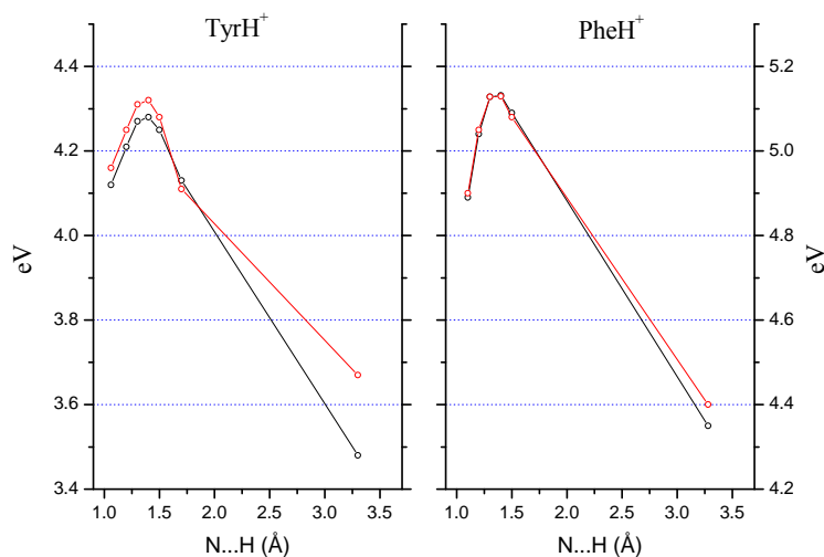
Figure 5: Minimum Energy Path (MEP) for the proton transfer reaction from the ammonium group to the aromatic ring for the stack (red line) and rot (black line) conformers of TyrH + ( syn ) (left) and PheH + (right). The last point at large N-H distance corresponds to the excited state energy of the transferred structures.
