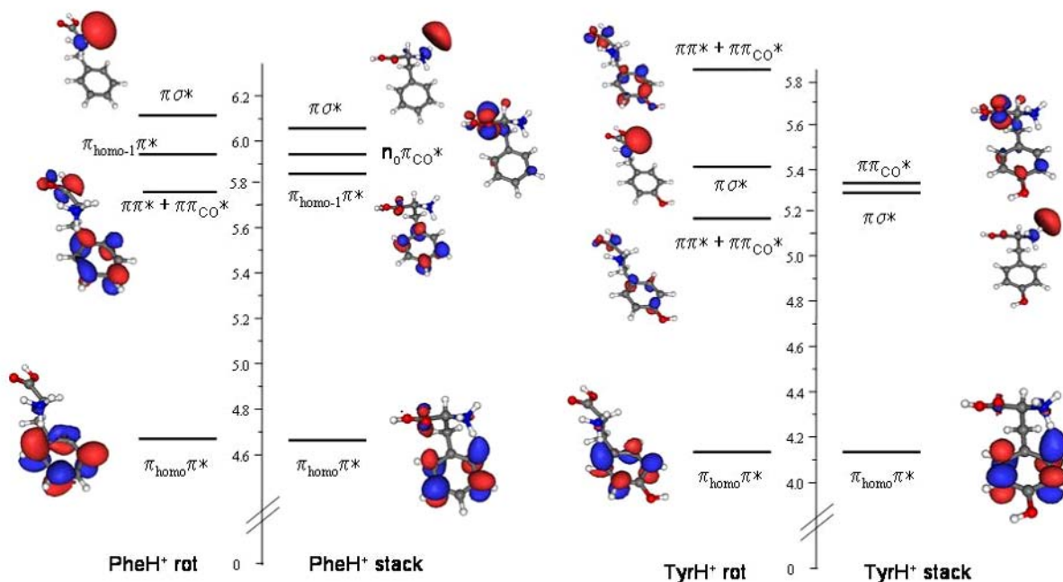
Figure 3: Excited state energies (CC2/aug-cc-pVDZ) along with the most contributing MO representation at the S_1 optimized structure for the rot and stack conformers of \text{PheH}^+ and \text{TyrH}^+ (syn orientation of the hydroxyl group).
