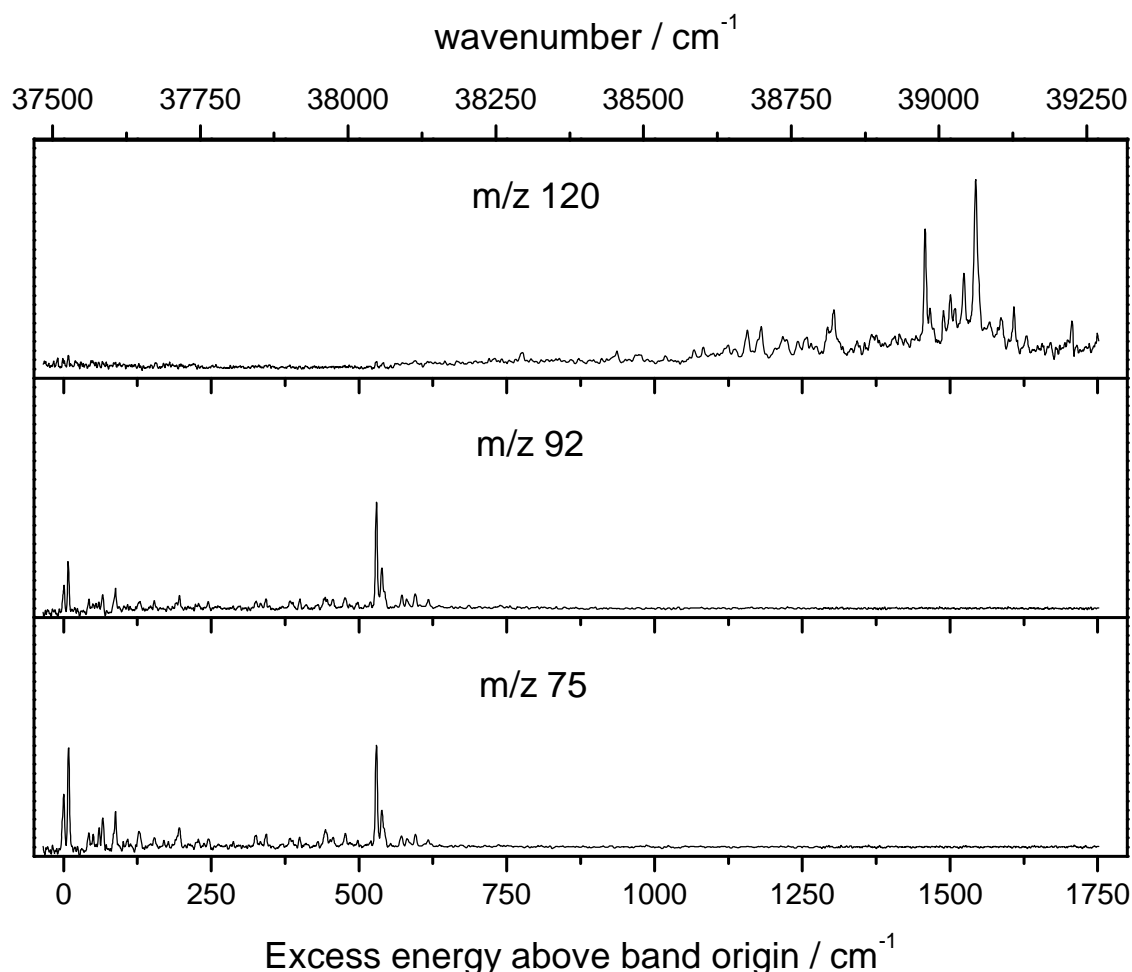
Figure 1: Photo-fragmentation spectra of protonated phenylalanine recorded on the three main fragmentation channels (same y axis scale) over a large spectral range: at low energies the fragmentation results in m/z 75 and m/z 92 following a proton transfer to the aromatic chromophore, while at higher energies these fragments disappear and m/z 120 is the only fragment produced.
