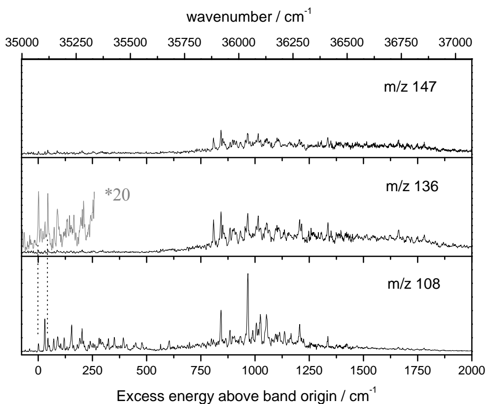
Figure 2: Photo-fragmentation spectra of protonated tyrosine recorded on the three main fragmentation channels (same y axis scale) over a large spectral range: at low energies the fragmentation results mainly in m/z 108, while at higher energies the m/z 147 and m/z 136 fragments become as intense as the former one. The spectra recorded on m/z 123 and m/z 119 fragments are not presented but they are similar to m/z 136 and m/z 147. The vertical dotted lines show positions of the origin and the first vibronic band at 43\text{ cm}^{-1} of the stack-syn conformer.
