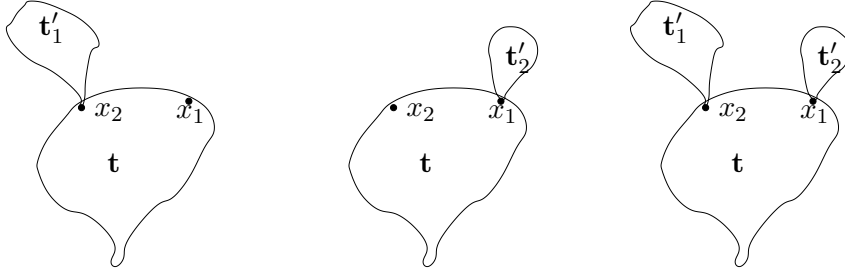
Figure 2.1: Exemple of the third case above. The trees are respectively \mathbf{t}_1, \mathbf{t}_2, \mathbf{t}_1 \cup \mathbf{t}_2 .
