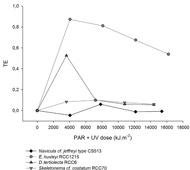
Fig. 3. Singlet oxygen transfer efficiency ( TE_{O_2} ) during PAR + UV irradiation ( \text{kJ m}^{-2} ) of senescent cells of Navicula cf. jeffreyi type (silica matrix), E. huxleyi (carbonaceous matrix), D. tertiolecta (no matrix) and Skeletonema cf. costatum (silica matrix).
