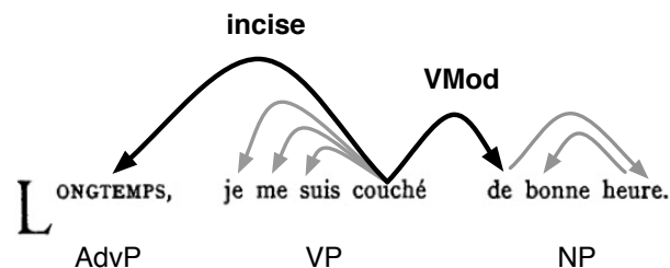
Fig. 4. Dependency structure of the sentence: "Longtemps, je me suis couché de bonne heure." ("For a long time I used to go to bed early"). Arrows represent dependencies: grey arrows, substitutions; and black arrows, adjunctions. Black arrows indicate the left adjunction of the adverbial phrase (AdvP) "longtemps" ("For a long time") as an incise to the verbal phrase (VP) "je me suis couché" ("I used to go to bed"), and the right adjunction of the nominal phrase (NP) "de bonne heure" ("I used to go to bed early") as a verb modifier to the verbal phrase (VP).
