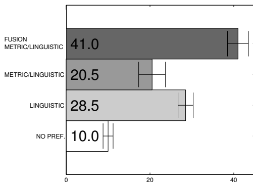
Fig. 6. Mean preference score and 95% confidence interval obtained for: the fusion of the linguistic/metric constraints, the linguistic/metric constraints, the linguistic constraint, and no preference.
