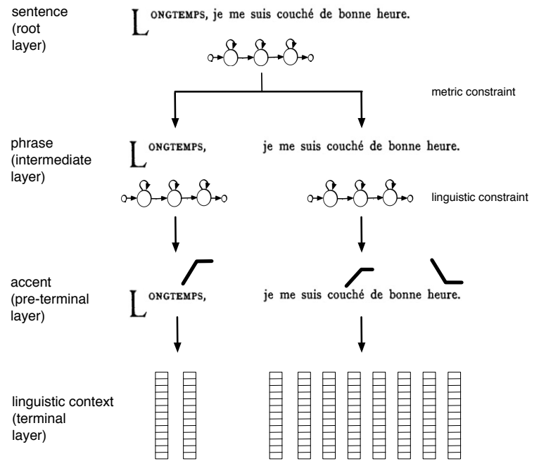
Fig. 5. Schematic illustration of the HHMM for the assignment of prosodic events.
