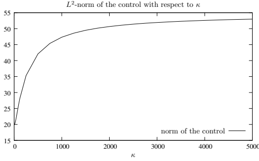
(a) Plot of the norm of the control with respect to \kappa .
