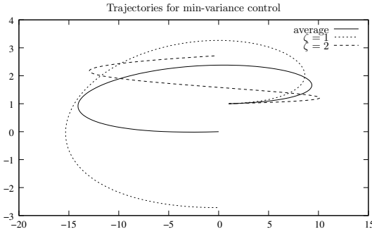
(a) Controlled trajectories in the phase plan using the optimal control for \kappa = 5 \cdot 10^3 . The variance at final time is 7.41.
