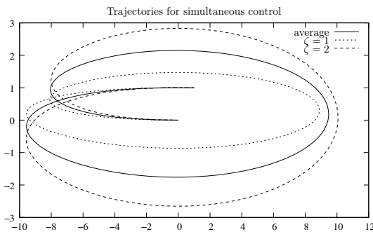
(a) Controlled trajectories in the phase plan using the simultaneous control.
