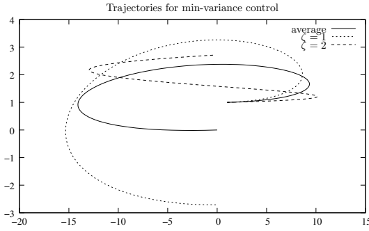
(a) Controlled trajectories in the phase plan using the optimal control for \kappa = 5.10^3 . The variance at final time is 7.41.
