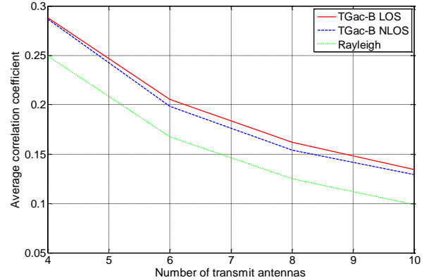
Fig. 7. Average correlation coefficient versus the number of transmit antennas
