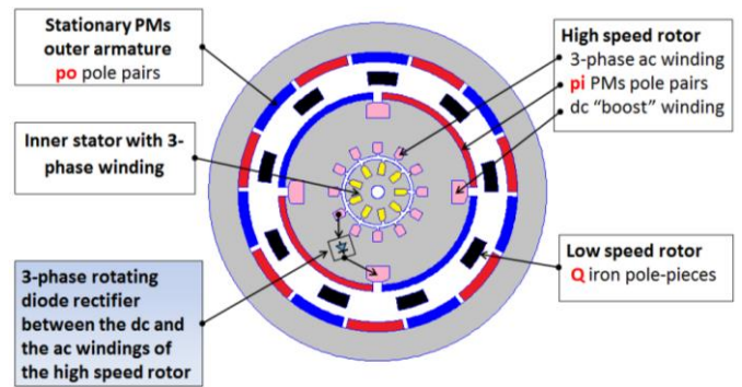
Fig. 1. 2D cross section view of MaGIM
