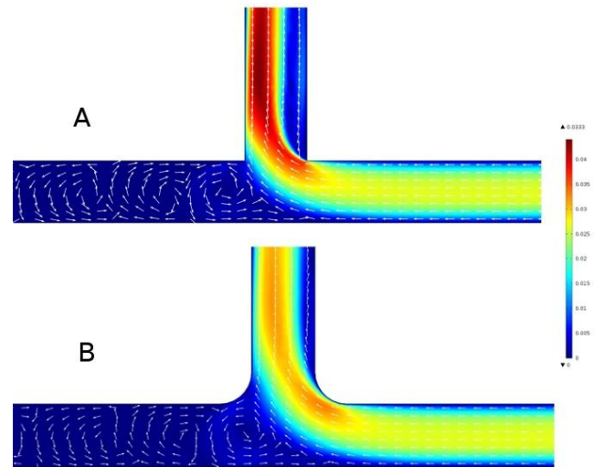
FIG 7: Influence of the curvature radius on the flow at a Tee-junction
