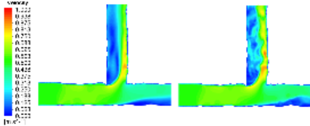
FIG 5: Comparison of turbulence simulation (velocity) using methods RANS (left) and LES (right).
