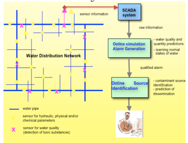
FIG 2: General system concept of SMaRT-Online WDN .
