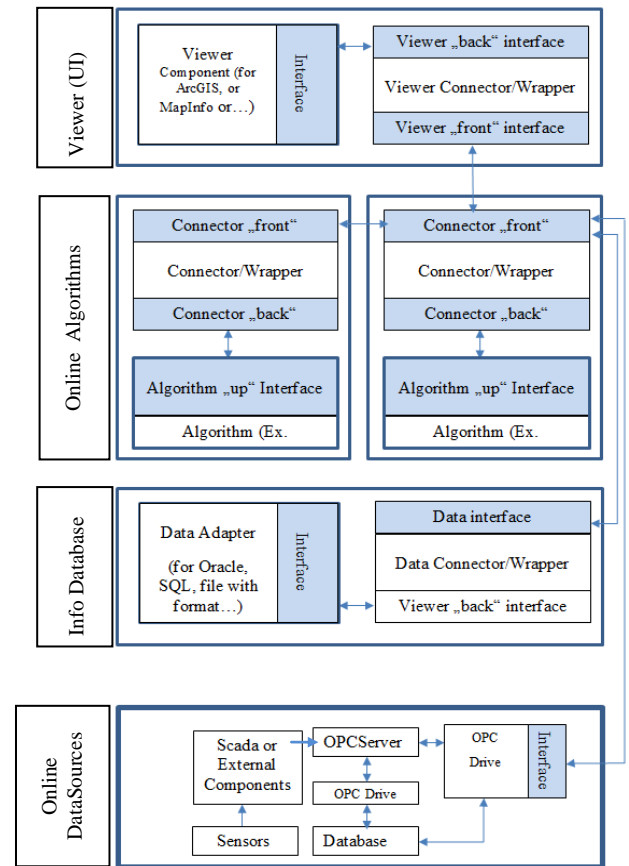
FIG 4: Abstract view of the software architecture for supporting online calculations.
