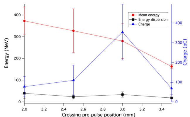
FIG. 3. Evolution of the mean energy (red circle), charge (blue triangle), and energy spread (black square) of electron spectra as a function of the crossing pre-pulse z position. Each point show the average over all the quasi-monoenergetic electrons beams.
