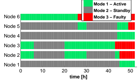
Fig. 3: Functioning modes of sensor nodes vs. time
