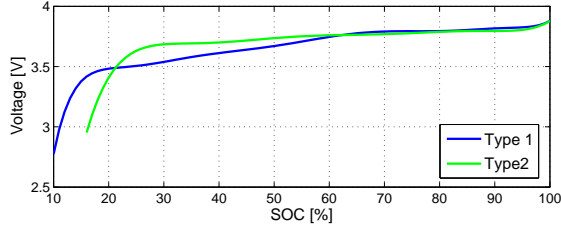
Fig. 2: SoC profiles for two battery types
