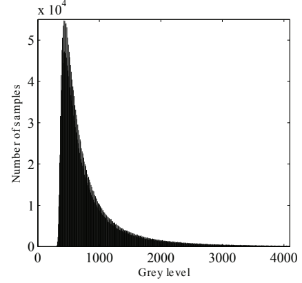
Fig. 2: Grey-level distribution.
