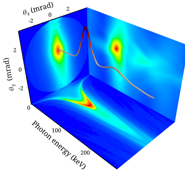
FIG. 4: Angular-spectral distribution of produced X-rays. Maps of the emission energy distributions d^2\varepsilon/d\omega d\Omega in the planes y = 0 (horizontal plane) and z = 0 (right vertical plane), and energy integrated angular distribution (left vertical plane). The angle \theta_y is angular distance along the y axis, while \theta_z is that along the z axis. The curve represents the on-axis spectral distribution. The calculation was performed for 600 MeV electrons.
