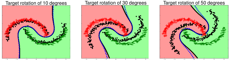
Figure 2: Decision boundaries of DALC on the intertwining moons toy problem, for fixed parameters B=C=1 , and a RBF kernel k(\mathbf{x}, \mathbf{x}') = \exp(-\|\mathbf{x} - \mathbf{x}'\|^2) . The target points are black. The positive, resp. negative, source points are red, resp. green. The blue dashed line shows the decision boundaries of algorithm PBDA (Germain et al., 2013).
