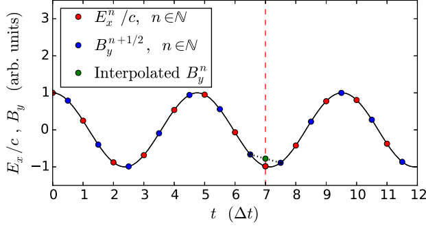
FIG. 7. Schematic evolution of the E_x and B_y fields for a sinusoidal wave, in a PIC simulation. On the Yee lattice, the discrete fields E_x^n/c (red dots) and B_y^{n+1/2} (blue dots) lie exactly on the same sinusoid. However, when interpolating the B_y field to an integer time (dashed red line), the interpolated field B_y^n is not on the sinusoid (green dot), and thus the E_x and B_y fields do not cancel exactly when computing the Lorentz force.
