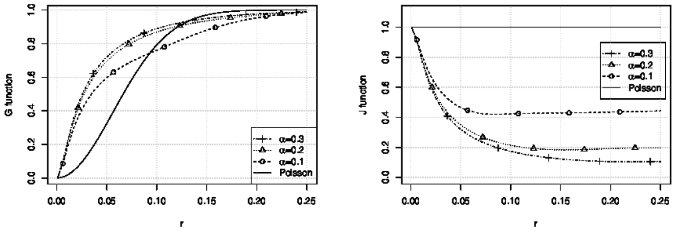
Figure 1: Laplace approximations of the G - (left) and J -functions (right) for three planar stationary LGCPs with intensity \rho = 50 and a spherical covariance function with variance \sigma^2 = 4 and scale parameters \alpha = 0.1, 0.2, 0.3 , respectively.
