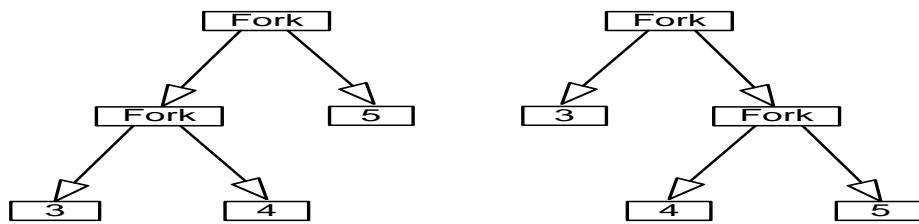
Two trees with the same fringe [3 4 5]
