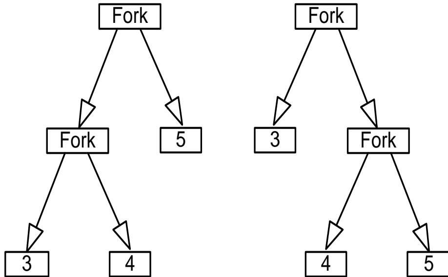
Two trees with the same fringe [3 4 5]
