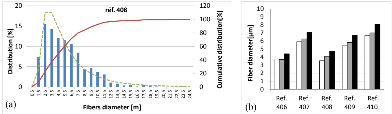
Fig. 3. Statistical representation of microstructural data. (a) Fiber diameters histogram (blue), associated cumulated distribution (red), and corresponding log-normal distribution (green). (b) Log normal mean (white), median (grey), arithmetic means (black) (b).
