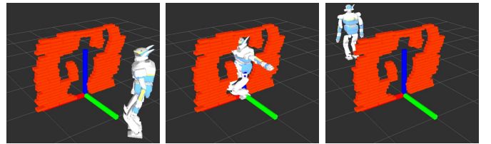
Fig. 16: Wall Motion Planning Problem. Left initial configuration Middle one irreducible configuration on the final trajectory found by an RRT on the irreducible subspace Right goal configuration. Adapted from [1].
