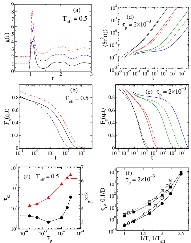
FIG. 1: Evolution of the structure and dynamics with the persistence time \tau_p at T_{\text{eff}} = 0.5 (a-c) and comparison of dynamics in active systems with \tau_p = 2 \times 10^{-3} and Brownian systems at T = T_{\text{eff}} = 0.5 (d-f). In (a,b) solid lines correspond to \tau_p = 0 (equivalent to a thermal system at T = 0.5 ), and the dashed, and dot-dashed lines correspond to \tau_p = 2 \times 10^{-3} , and 2 \times 10^{-2} , respectively. In (a) we show the pair distribution function g(r) ; the curves are shifted vertically for clarity. In (b) we show the self-intermediate scattering function F_s(q; t) = \langle e^{i\mathbf{q} \cdot (\mathbf{r}_j(t) - \mathbf{r}_j(0))} \rangle for q = 7.25 . In (c) we show the relaxation time, \tau_\alpha (circles) and the peak value of g(r) (triangles). The relaxation time is defined as F_s(q; \tau_\alpha) = e^{-1} . In (d,e) solid lines correspond to active systems at T_{\text{eff}} = 1, 0.6, 0.45 and 0.4 , and dashed lines correspond to equilibrium systems at T = 1, 0.6 and 0.45 (from left to right). In (d) we show mean-square displacement \langle \delta r^2(t) \rangle = \langle (\mathbf{r}_j(t) - \mathbf{r}_j(0))^2 \rangle and in (e) we show F_s(q; t) . In (f) circles represent \tau_\alpha , squares represent the inverse self-diffusion coefficient, 0.1/D of active (closed symbols) and thermal (open symbols) systems.
