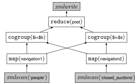
Fig. 1. Outline of the PACT program generated by PAXQuery for the XQuery in Example 1.
