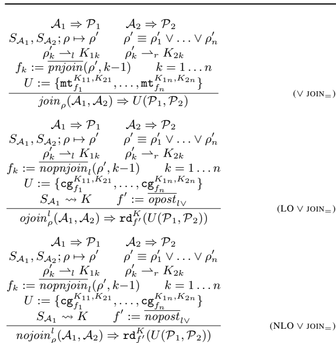
Fig. 13. Disjunctive equi-join translation rules.
