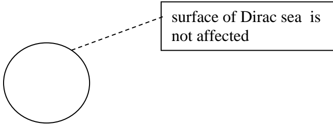
Fig. 13.1 No vortices ( \exists superconductivity).
