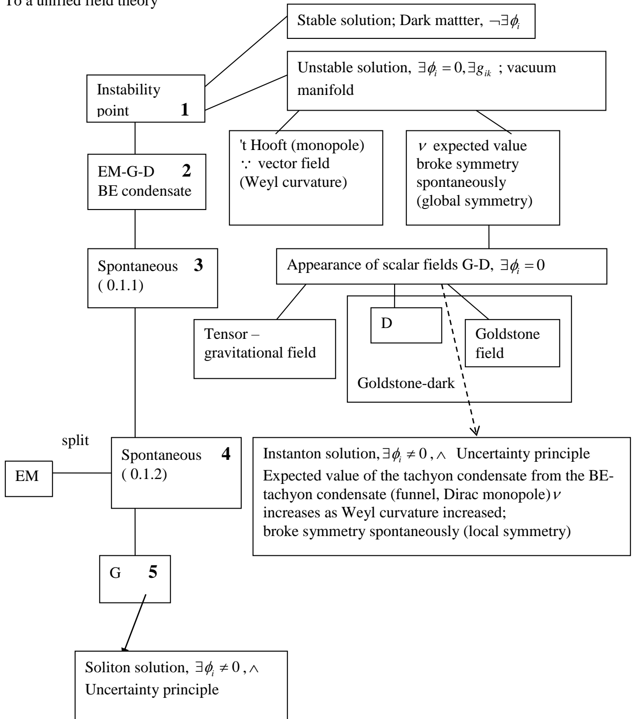
Fig. 6 Ref. Symmetry breaking mechanism and eq. (1.1 b) (EM: electromagnetic field, D: dark field, G: gravitational field).
