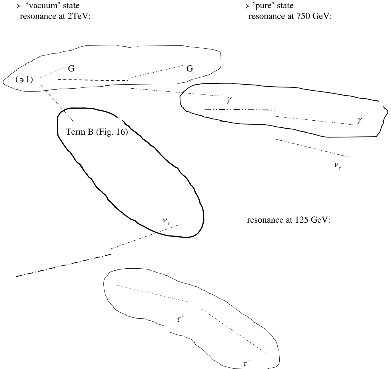
Fig. b) Dark boson decay properties (restoring path):
