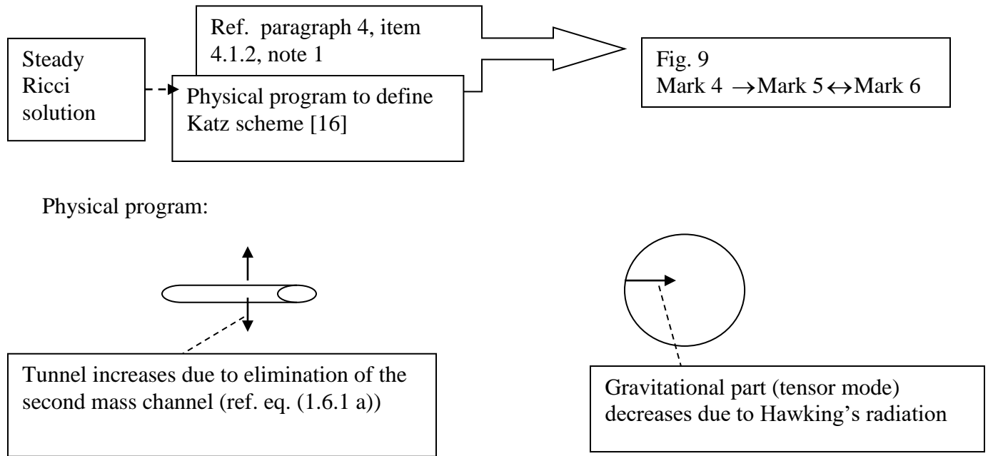
Fig. 10.4 Tunnel-gravitational part dynamics (step 4).
