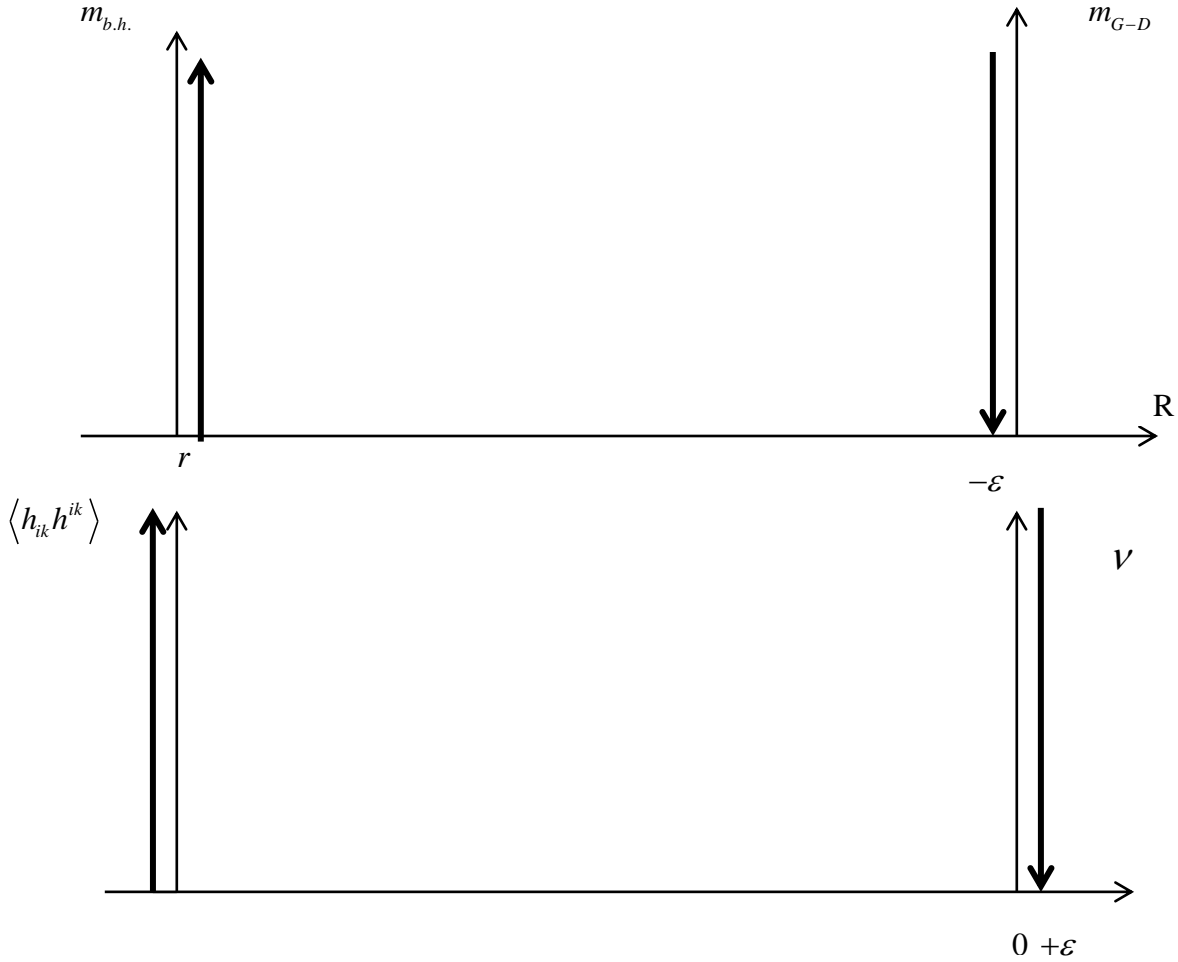
Fig. 7 Corollary of instanton solution (\phi_i = 0, \forall x \in [r, 0[; \phi_i \neq 0, \forall x \in [0, R[ ]) ; by dint of a), b).
