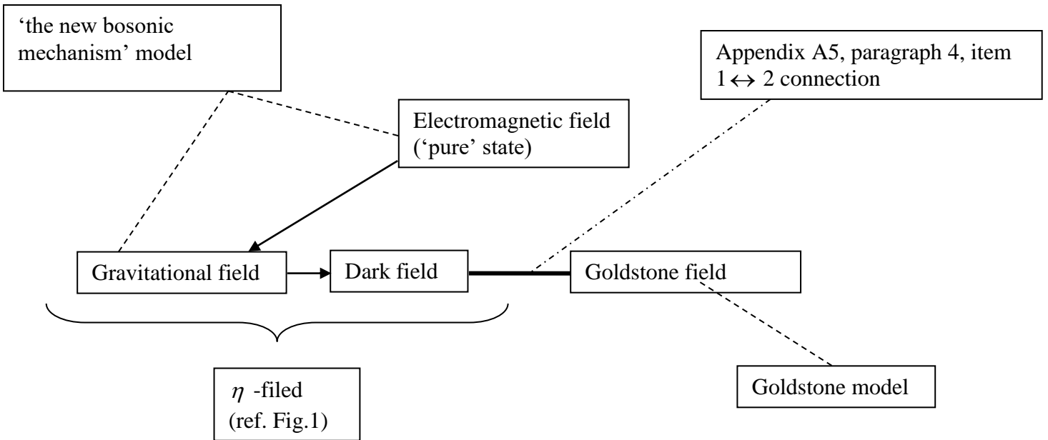
Fig. 1.2 Correspondence to ‘the new bosonic mechanism’ (theory framework).
