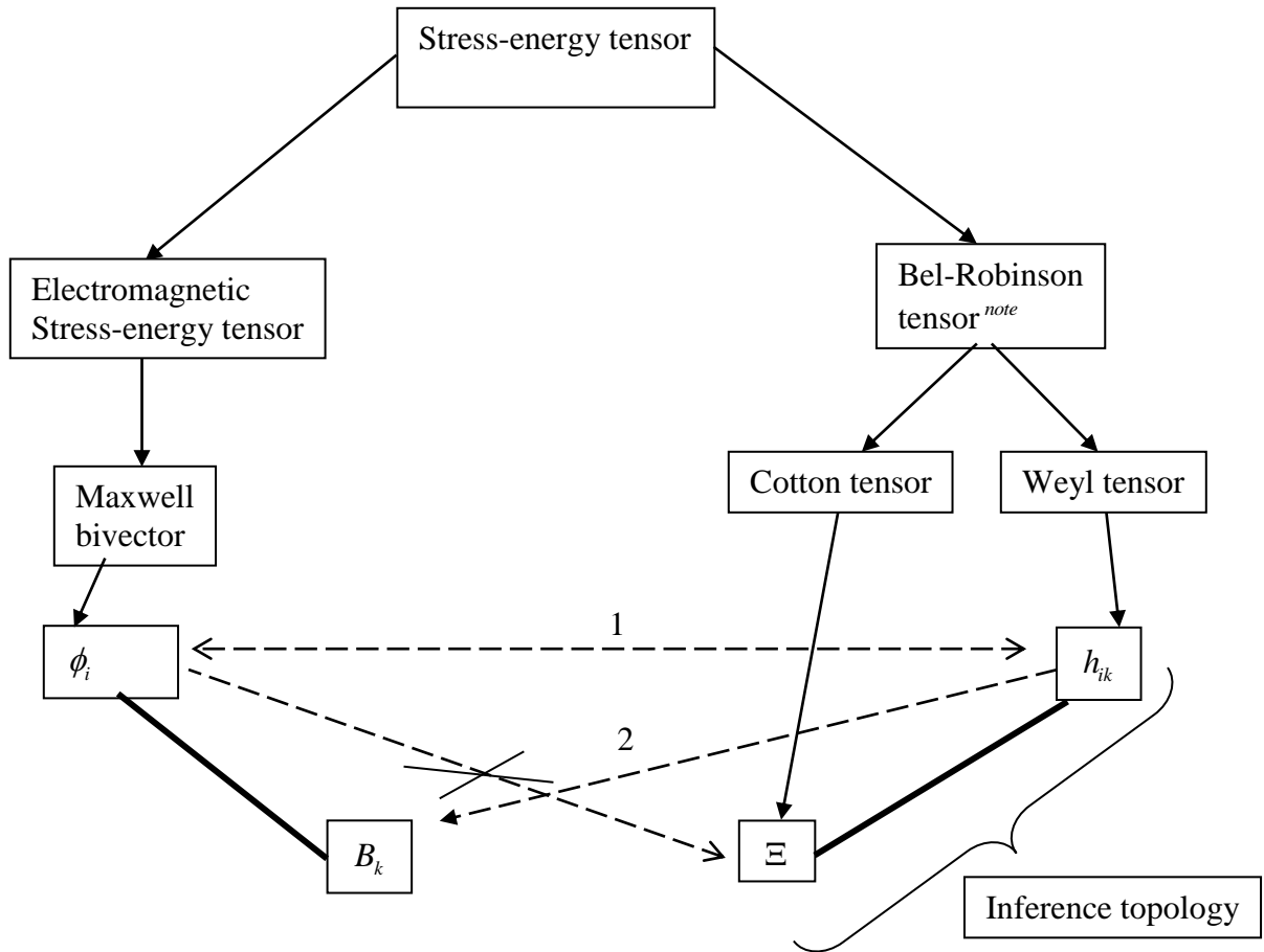
Fig. 8.2 Coupling due to h - tensor-graviton.
