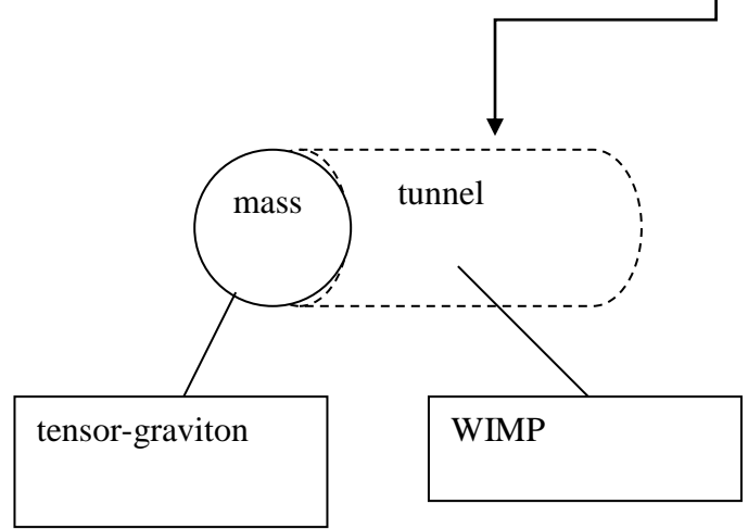
Fig. TF-1.3 Coupling due to h - tensor-graviton.
