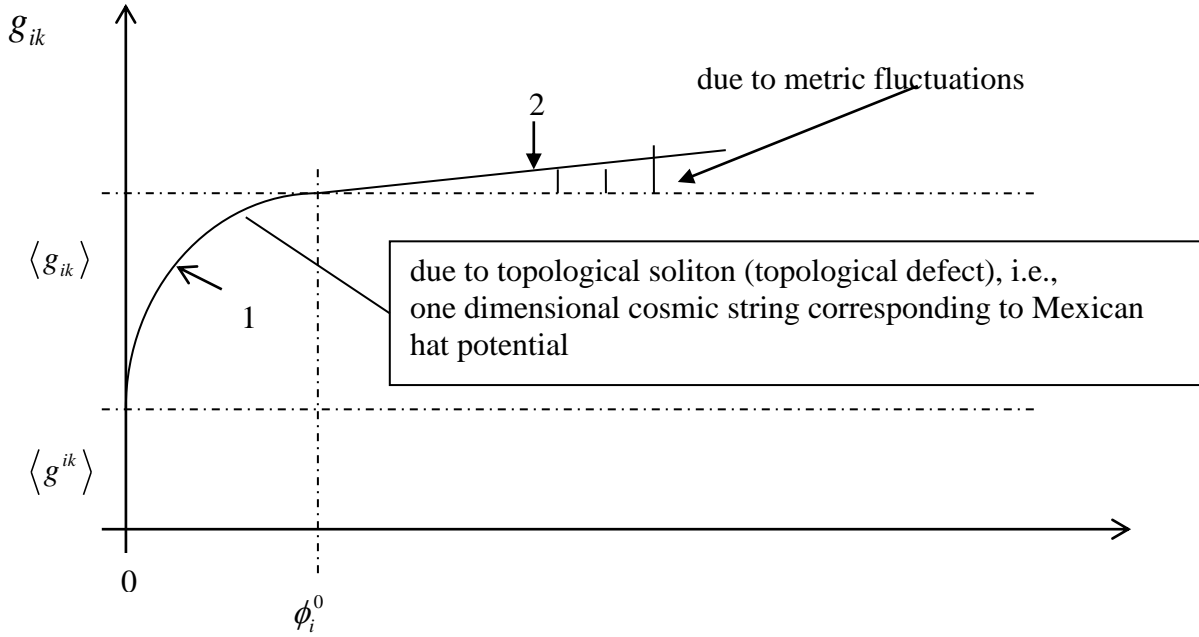
Fig. 4 Metric tensor as a representation by the power law function (\phi^i)^n
