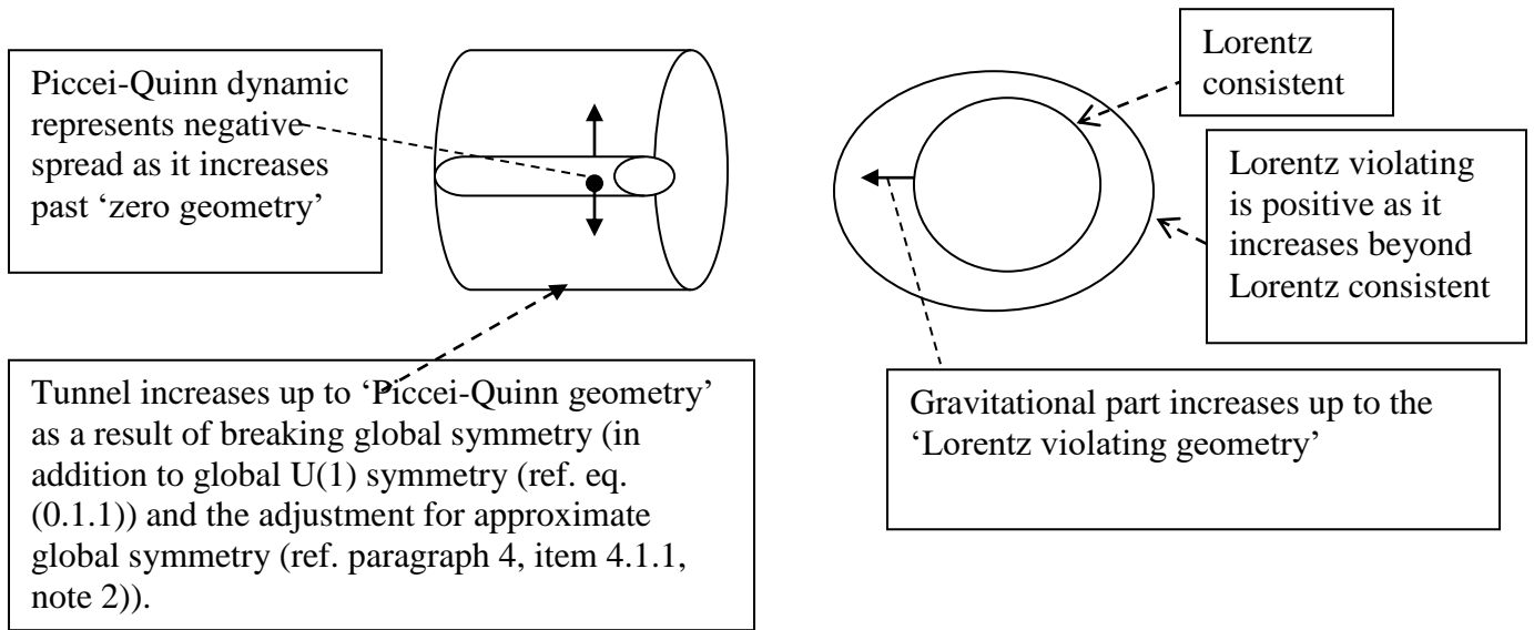
Fig. 10.3 Tunnel- gravitational part dynamics (step 3).
