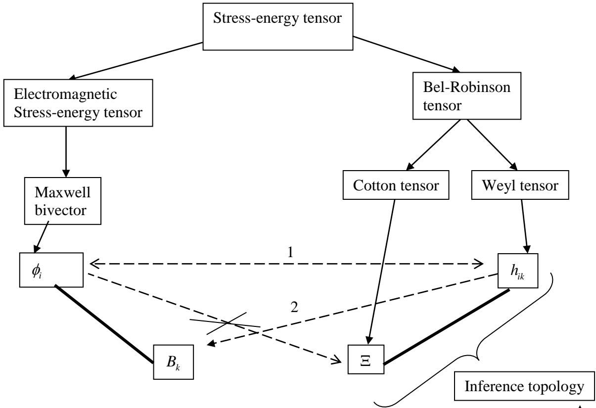
Fig. TF-1.3 Coupling due to h - tensor-graviton.
