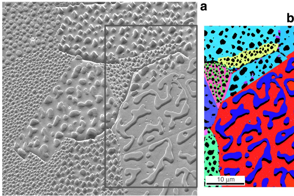
Figure 3: (a) Secondary electron image of a region with nine Ni grains and their associated Ag crystals. This image has been corrected for sample tilt in the microscope. (b) Orientation map of the outlined portion of (a). At the bottom right, a Ni(100) grain (red) can be recognized by its meandering finger-like Ag(111) crystals (blue). On most of the other Ni grains, the color of the Ag crystals is close to that of the underlying Ni grain, and the black regions next to each Ag grain are unidentifiable because of shadowing by the Ag crystals due to sample tilt [18, 22].
