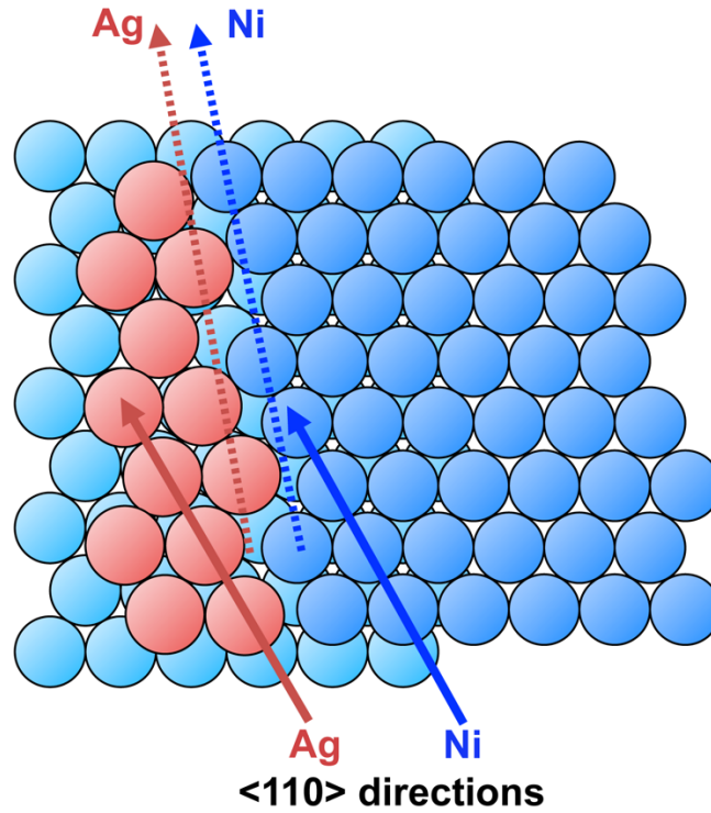
Figure 7 : Schematic top view of step on high-index Ni surface (Ni atoms blue) with Ag atoms (red) attached to the step edge. The arrows indicate step directions and close packed directions in both the Ni substrate and the Ag atoms attached to the step.
