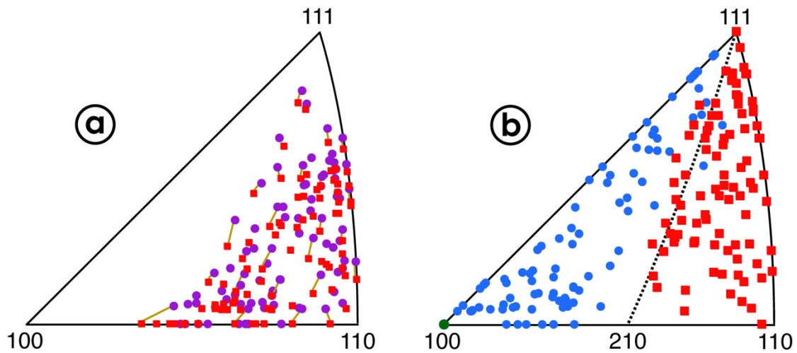
Figure 5: (a) Ag crystal orientations (square red symbols) that display a cube-on-cube OR to the Ni substrate (round purple symbols as in Fig. 4a); (b) Ag orientations that display OR(S) on the Ni substrate (round blue and green symbols as in Fig. 4a). The dashed line from (111) to (210) represents the [1\bar{2}1] zone.
