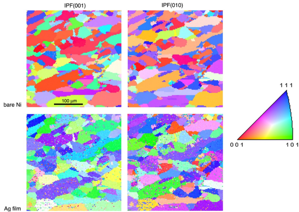
Figure 1: Inverse pole figure (IPF) maps of grains of the same region of a sample in two perpendicular directions of the microscope reference frame. The top panels correspond to the bare Ni substrate, and the bottom panels to the Ag deposit on Ni; the orientation color code is given in the SST on the right (color on line).
