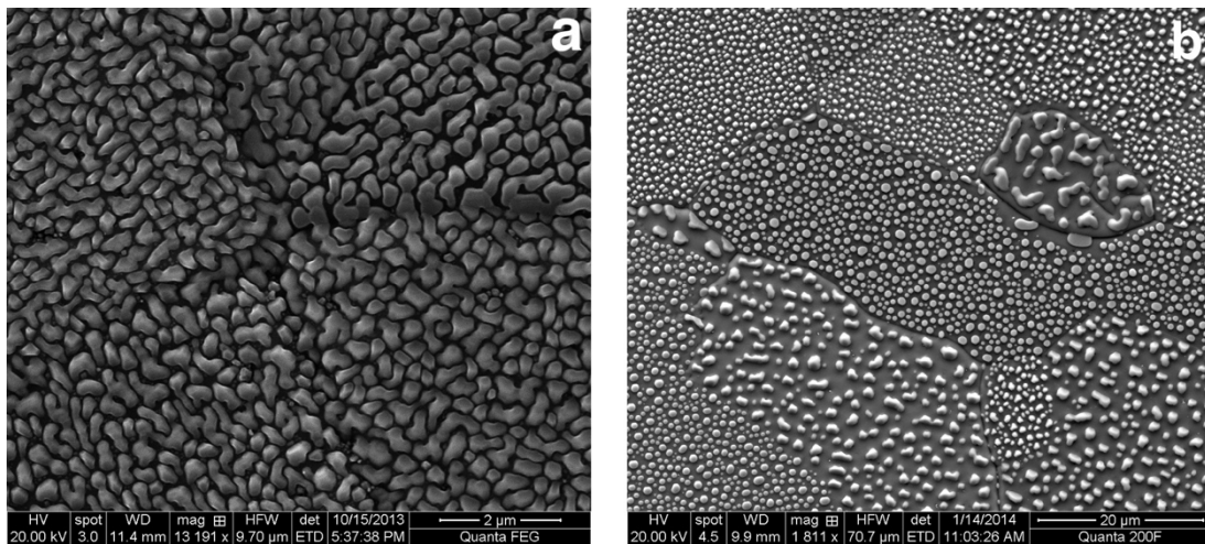
Figure 2: (a) SEM micrograph of Ag film microstructure after deposition at 413 K. Top view of five grains. (b) SEM micrograph of Ag crystals on the Ni grains after annealing at 923 K for 2 h. Note the different dispersions and sizes of Ag crystals residing on Ni grains of different orientations.
