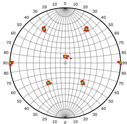
Figure 3. Example to illustrate the method used to determine the orientation of Ag deposit films after MD simulation and relaxation. The figure shows a projection of Ag nearest neighbor vectors onto a stereographic projection for the case of an Ag film equilibrated on Ni(511), to yield a \langle 110 \rangle pole figure of the Ag deposit. Small red points show the scatter of poles obtained from 500 Ag atoms in the deposit. Large green points represent the average positions of the red points (color on line). The computed Ag film interfacial plane orientation is approximately (331).
