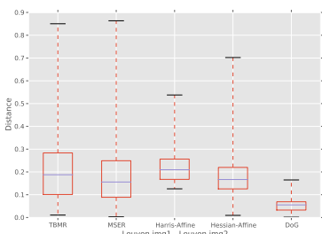
(a) Leuven img1 - img2.
