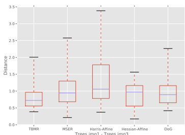
(b) Trees img1 - img3.
