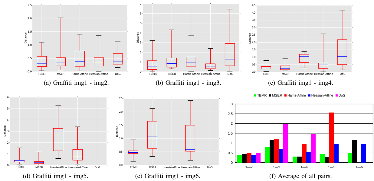
Fig. 10. Distributions of errors in image registration by homography on “Graffiti” image pairs, which comes with a ground truth. DoG fails registering pairs (1,5) and (1,6); Harris-Affine fails on (1,6). There is a slight advantage for MSER on pair (1,5), while on all other pairs TBMR performs better.
