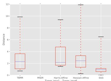
(e) Trees img1 - img6.
