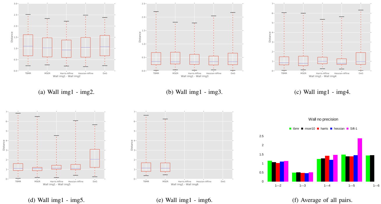
Fig. 9. Distributions of errors in image registration by homography on “Wall” image pairs, which comes with a ground truth. Harris-Affine, Hessian-Affine, and DoG fails registering pairs (1,6); TBMR performs similar with MSER on all the pairs and similar with Harris-Affine, and Hessian on all other pairs than (1,6). In general, TBMR performs better than DoG on all the other pairs.
