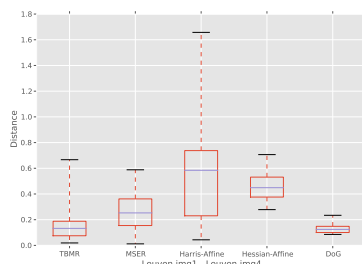
(c) Leuven img1 - img4.
