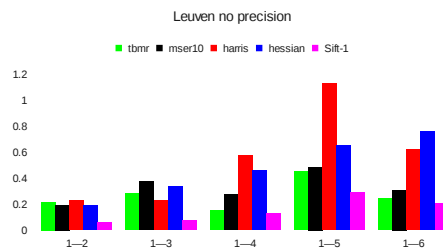
(f) Average of all pairs.
