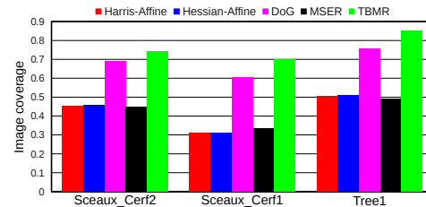
Fig. 8. Image coverage evaluation by dilating a keypoint with a 2D window having size 31 \times 31 ; Vertical axis represents the average rate of area covered by the dilated region for multi-view images presented in Fig. 5, Fig. 17, and Fig. 18.
