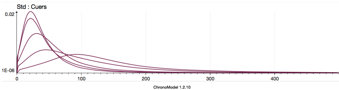
FIGURE 9. Cuers, Ex 2 (Cont.) Posterior densities obtained for standard deviations \sigma_i .
