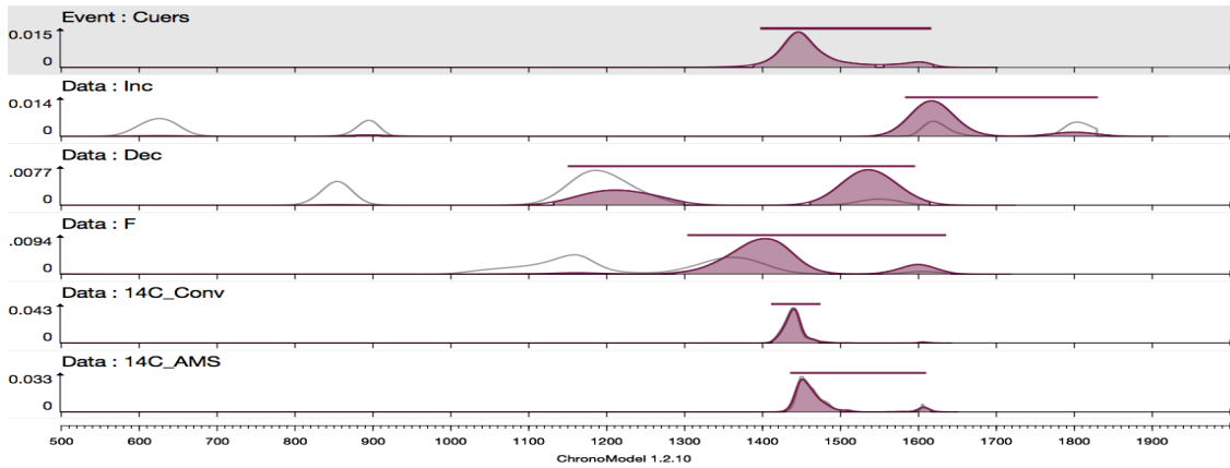
FIGURE 8. Cuers, Ex. 2. Posterior density of the event date \theta (gray background). Posterior densities of t_i (red line & white background) and individual posterior calibrated densities (gray line & white background) obtained for archaeomagnetic and ^{14}\text{C} dates.
