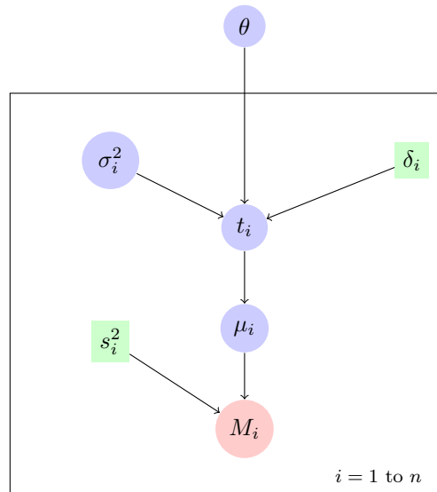
FIGURE 11. DAG for the wigggle matching model.
