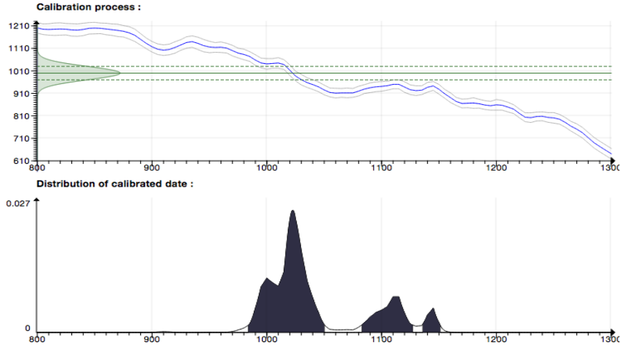
FIGURE 1. Conversion of a ^{14}\text{C} age ( A = 1000 \pm 30 BP) to a calendar date via the calibration curve IntCal13.
