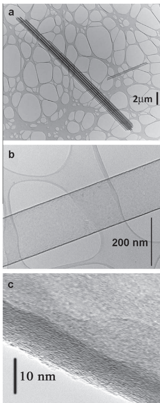
Fig. 9 – TEM-HRTEM images of carbon nanotubes (sample M18).
