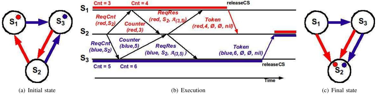
Figure 3. Execution example
