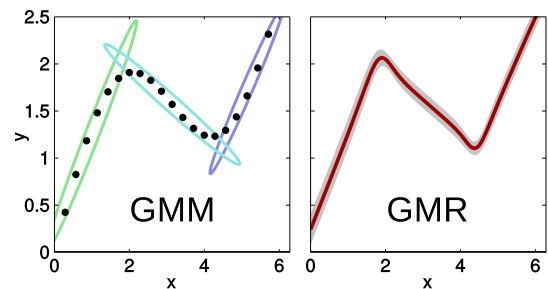
Figure 11: Left: Gaussian Mixture Model (GMM) with 3 Gaussians on the 20 example data points. This model is acquired through unsupervised learning on the joint input×output space. Right: Gaussian Mixture Regression, which yield the mean and variance in the output space Y when conditioning on the input space X .
