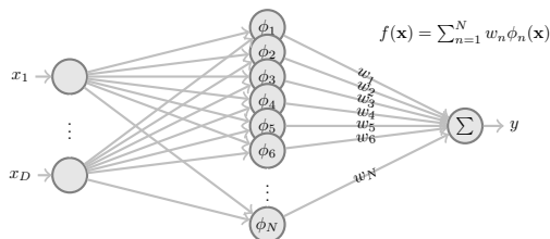
Figure 14: The function model used in KRR as a network.
