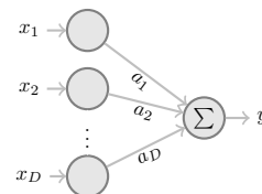
Figure 4: Network representation of a linear model.
