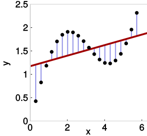
Figure 5: Illustration of least squares. Black dots represent the training examples, and the thick line is the learned function f(\mathbf{x}) . Vertical lines represent residuals.
