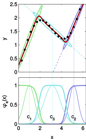
Figure 12: Relationship between GMM and the unified model. The basis functions are the (normalized) projections of the Gaussians in the GMM on the input space. The linear models have slopes a_e = \Sigma_{e,YX} \Sigma_{e,Y}^{-1} and offsets b_e = \mu_{e,Y} - \Sigma_{e,YX} \Sigma_{e,X}^{-1} \mu_{e,X} .
