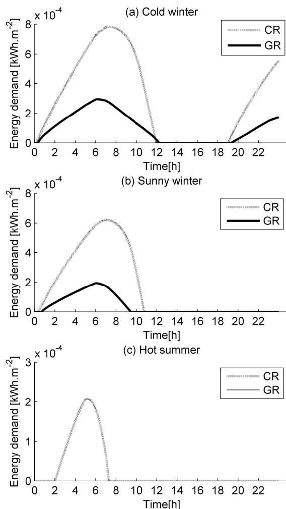
Figure 9. Minimum energy demand for conventional (CR) and green (GR) roofs in Antananarivo: (a) cold winter; (b) sunny winter; and (c) hot summer.
