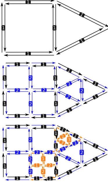
Figure 6: Edge labels are used as a guide to reconstruct \phi_1^i relations. Only three different labels are needed to be able to distinguish an original edge from all edges connected to it during the refinement steps.
