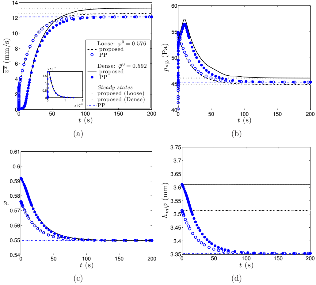
Figure 5: Low viscosity case: simulated (a) solid velocity \overline{v^x} , (b) solid pressure p_{s|b} , (c) volume fraction \bar{\varphi} , and (d) h_m \bar{\varphi} . Horizontal dotted and dash-dotted lines represent the limit steady states. The relative velocity \overline{v^x} - \overline{u^x} is plotted in the insert of figure (a) (also in mm/s).
