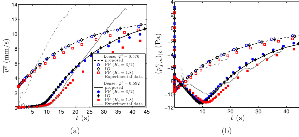
Figure 9: Low viscosity case: solid velocity \overline{v^x} and basal excess pore pressure (p^e_{fm})_b for times t \in [10^{-2}\text{s}, 45\text{s}] , for the proposed model, the Pailha-Pouliquen model (with K_4 = 3/2 and K_4 = 1.8 ), the Iverson-George type model and the experimental data.
