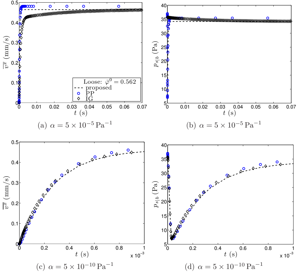
Figure 7: High viscosity case and small times: simulated (a,c) solid velocity \overline{v^x} and (b,d) solid pressure p_{s|b} , with \alpha = 5 \times 10^{-5} \text{ Pa}^{-1} for (a,b), and \alpha = 5 \times 10^{-10} \text{ Pa}^{-1} for (c,d). The results are shown for the proposed model (dashed lines), the Pailha-Pouliquen model (circles) and the Iverson-George type model (diamonds).
