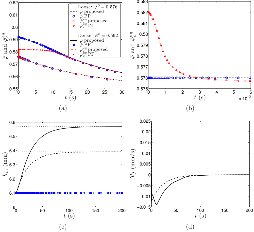
Figure 6: Low viscosity case: simulated (a-b) volume fraction \bar{\varphi} and critical volume fraction \bar{\varphi}_c^{eq} given by (5.8), (a) and (b) represent a zoom of figure 5c during the first 30s and at the very beginning of the simulation t \in [0, 0.006\text{s}] , respectively; (c) mixture thickness h_m ; (d) mass transfer \mathcal{V}_f .
