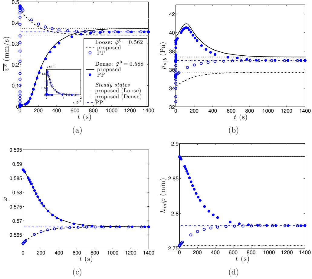
Figure 3: High viscosity case : simulated (a) solid velocity \bar{v}^x , (b) solid pressure p_{s|b} , (c) volume fraction \bar{\varphi} , and (d) h_m \bar{\varphi} . Horizontal dotted and dash-dotted lines represent the limit steady states. The relative velocity \bar{v}^x - \bar{u}^x is plotted in the insert of figure (a) (also in mm/s).
