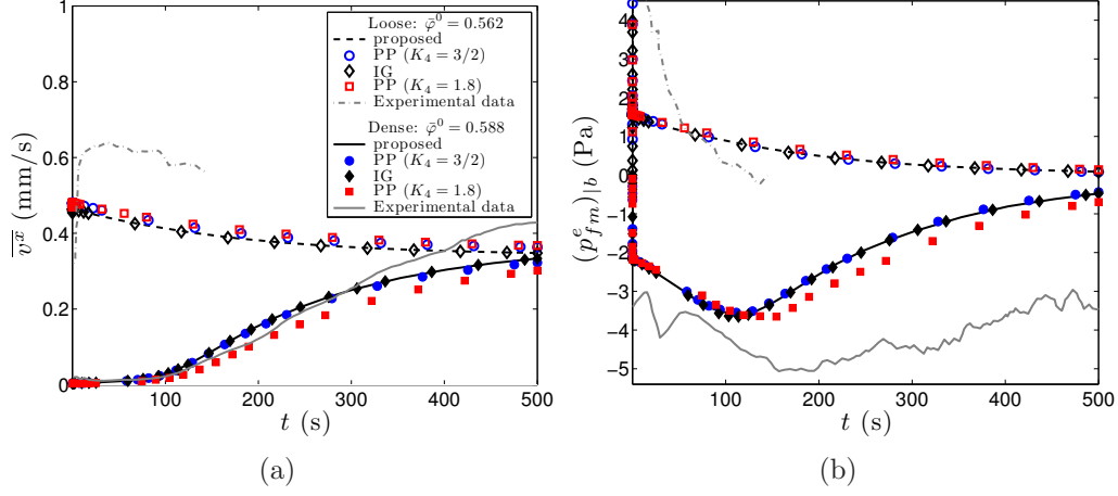
Figure 8: High viscosity case: solid velocity \overline{v^x} and basal excess pore pressure (p_{fm}^e)_b , for times t \in [10^{-3}\text{s}, 500\text{s}] , for the proposed model, the Pailha-Poulighen model (with K_4 = 3/2 and K_4 = 1.8 ), the Iverson-George type model and the experimental data.
