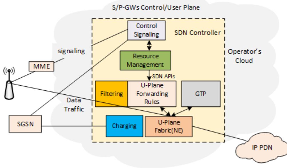
Figure 5. 6: Fully virtualized SDN-enabled cellular network
