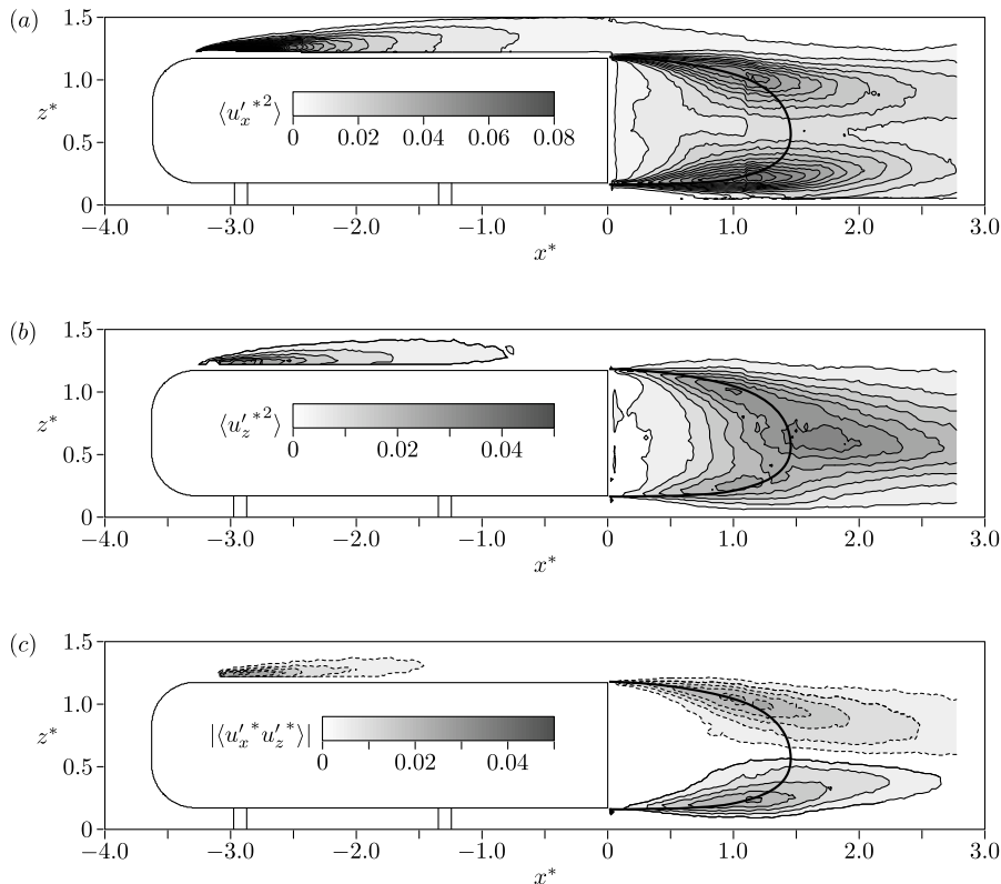
FIGURE 6. Contours of Reynolds stresses in the plane y^* = 0 : \langle u_x'^*{}^2 \rangle , (a); \langle u_z'^*{}^2 \rangle , (b); |\langle u_x'^* u_z'^* \rangle| , (c). Continuous and dashed lines are respectively positive and negative values, contour intervals are 0.005, contour 0 is not plotted. The thick black line represents the separatrix of the mean flow.
