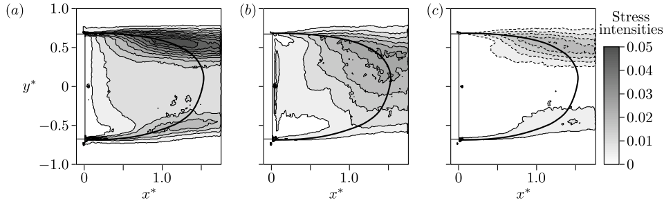
FIGURE 12. Contours of Reynolds stresses in the plane z^* = 0.6 of the wake in the #P state: \langle u_x'^2 \rangle , (a); \langle u_y'^2 \rangle , (b); \langle u_x' u_y' \rangle , (c). Continuous and dashed lines are respectively positive and negative values, contour intervals are 0.005, contour 0 is not plotted. The thick black line represents the separatrix of the mean flow of the #P state.
