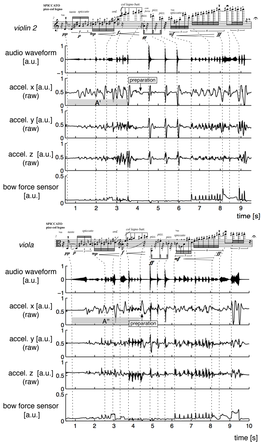
Figure 5: Score, audio waveform and sensor data for the prototypic phrase called spiccato . Top version was recorded by the second violin. Bottom version was recorded by the viola (transposed score). The gyroscope data were removed from the figure for clarity.
