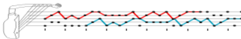
Figure 2. A limanza sequence with n = 30 , p = 6 .
