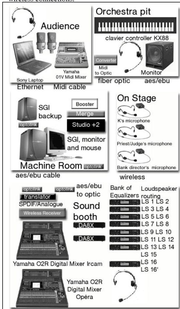
Figure 2. Hardware connections in K...
