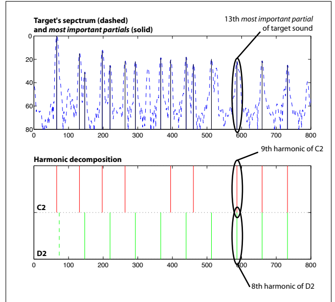
Figure 4. Harmonic decomposition of a target's most important partials . The target sound is a mixture of a contra-bass playing a C2 and a horn playing a D2.
