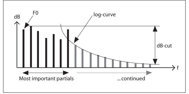
Figure 3. "Reconstruction" of the target's spectrum from its most important partials and F0s features. The log-curve and dB-cut parameters are determined through an optimization process in such a way that the spectral moments of the synthesized sound equal the original target's ones.
