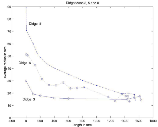
Figure 2 : Average internal radius of three didgeridoos.
