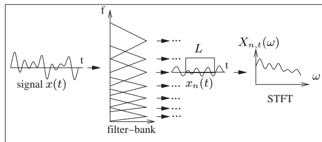
Figure 3: Features extraction from signal. From left to right: signal, filter bank, output signal of each filter, STFT of the output signals
