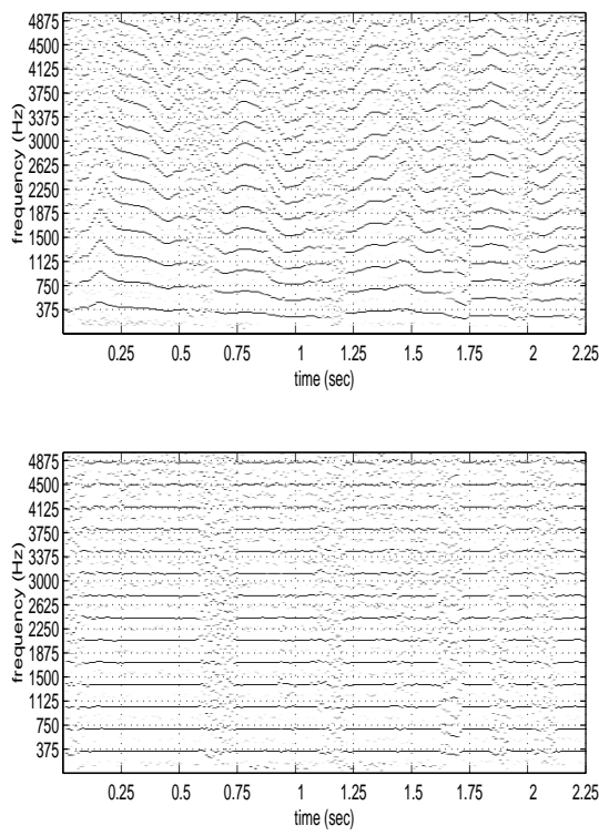
Figure 1: 1 - \Gamma(\omega, t) computed on a) original signal, b) pre-processed signal. Darker values indicate \Gamma(\omega, t) close to 1. Signal : Tibetan female singing voice ( \bar{f}_0(t)=345 Hz, LPC order 40, Blackman-Harris-3 window, 20ms)
