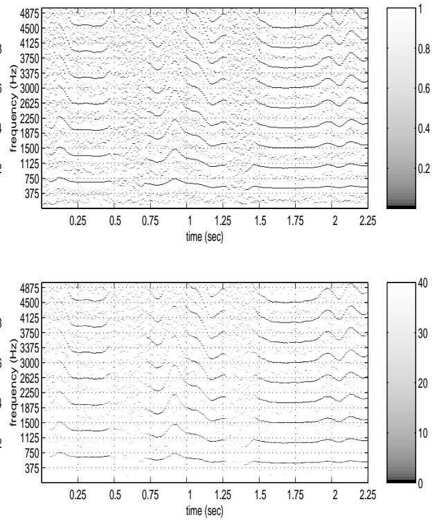
Figure 2: Sinusoidality estimation by a) \Gamma(\omega, t) , b) e(\omega, t)/f with frequency reassignment. Signal : Chinese female singing voice ( \bar{f}_0(t)=565 Hz, Blackman-Harris-3 window, 20ms, d=3.3 ms)
