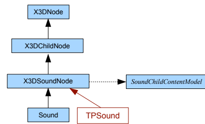
Figure 3: The proposed element TPSound extending X3DSoundNode .
